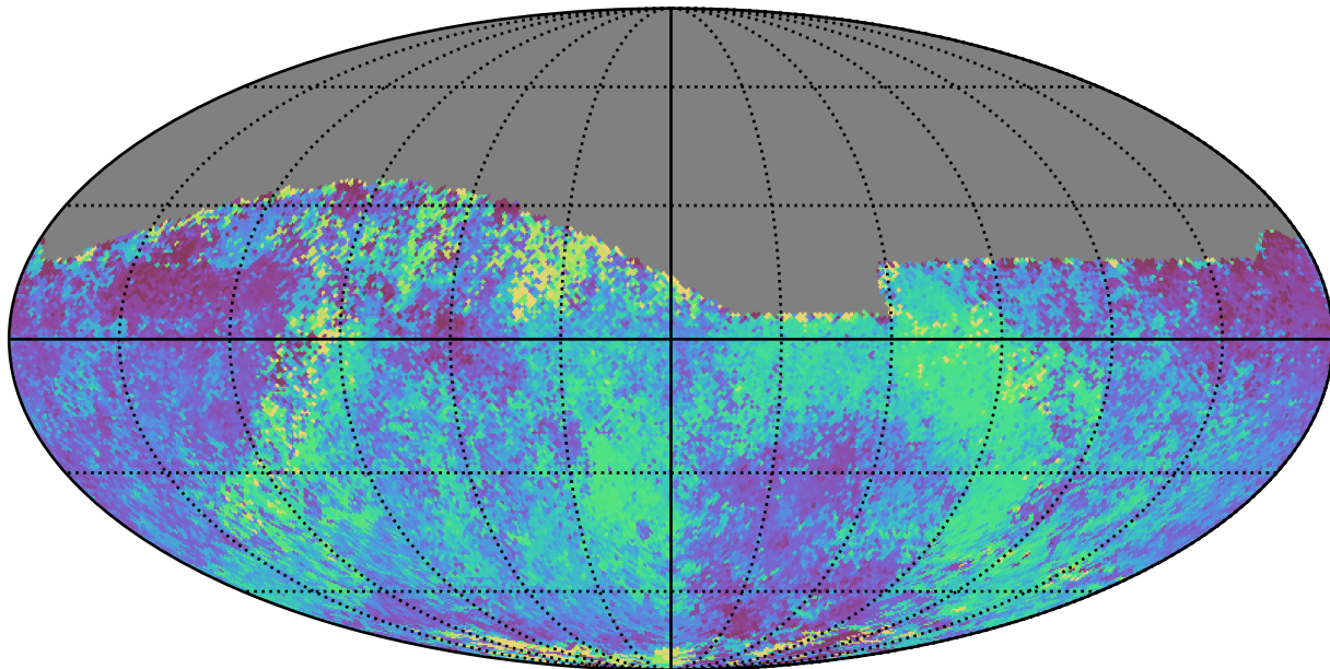
noroll_mjdp180_v3.4_10yrs Yr 1 all bands: Median skyBrightness
