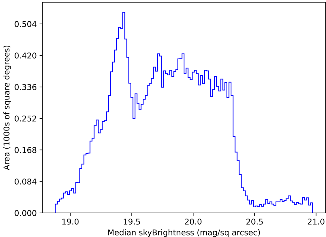
noroll_mjdp180_v3.4_10yrs Yr 1 all bands: Median skyBrightness
