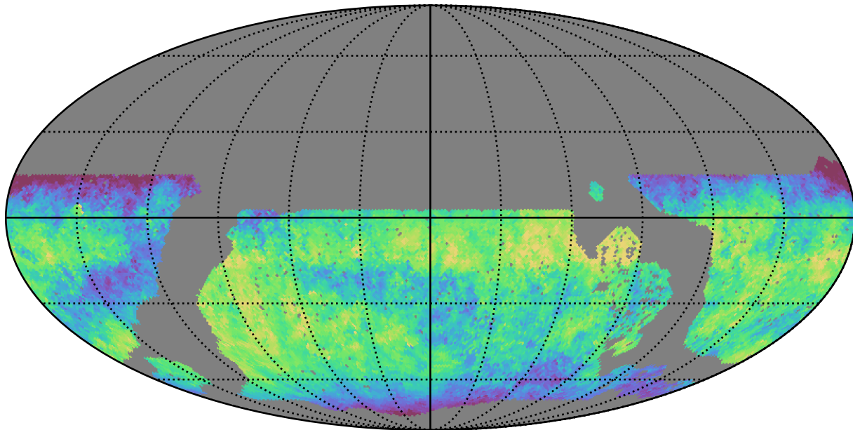
noroll_mjdp180_v3.4_10yrs WFD z band: Median skyBrightness
