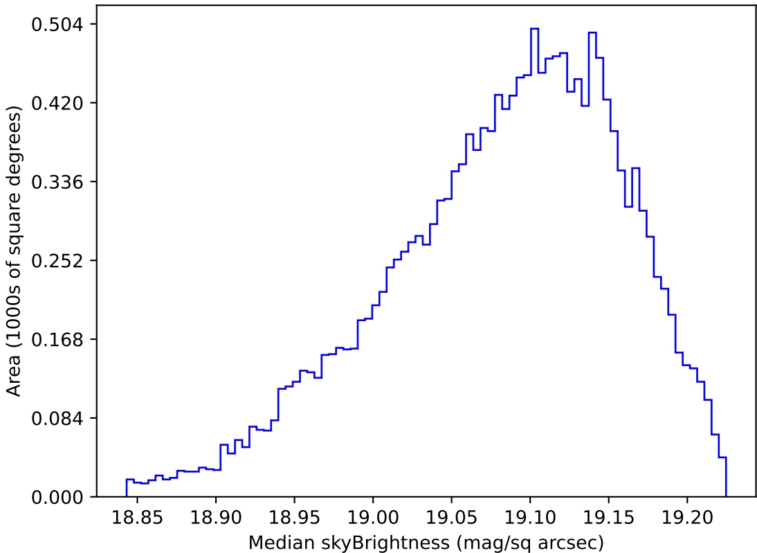
noroll_mjdp180_v3.4_10yrs WFD z band: Median skyBrightness
