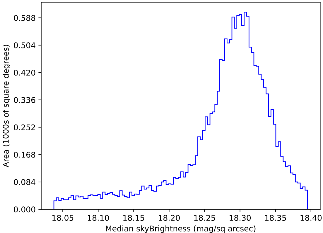
noroll_mjdp180_v3.4_10yrs WFD y band: Median skyBrightness
