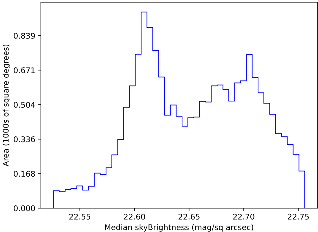
noroll_mjdp180_v3.4_10yrs WFD u band: Median skyBrightness
