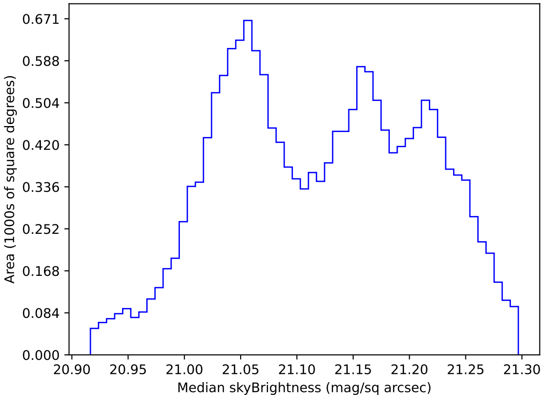
noroll_mjdp180_v3.4_10yrs WFD r band: Median skyBrightness
