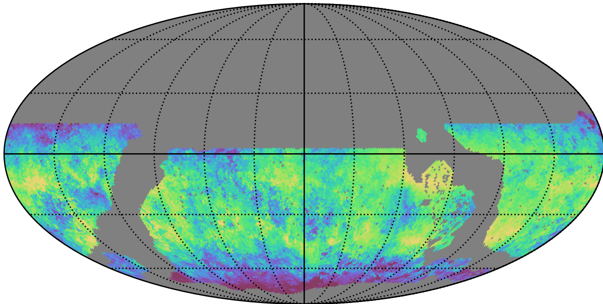
noroll_mjdp180_v3.4_10yrs WFD i band: Median skyBrightness
