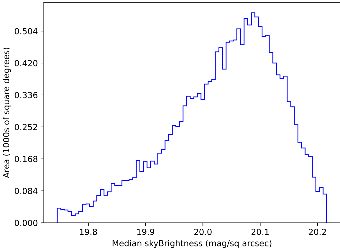
noroll_mjdp180_v3.4_10yrs WFD i band: Median skyBrightness
