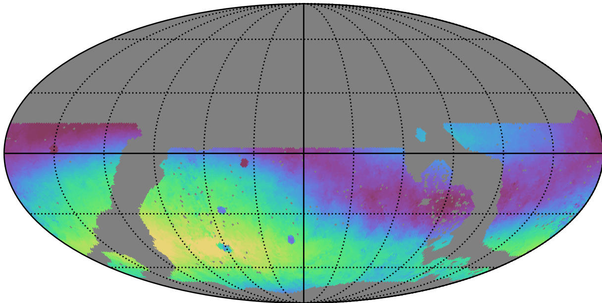
noroll_mjdp180_v3.4_10yrs WFD g band: Median skyBrightness
