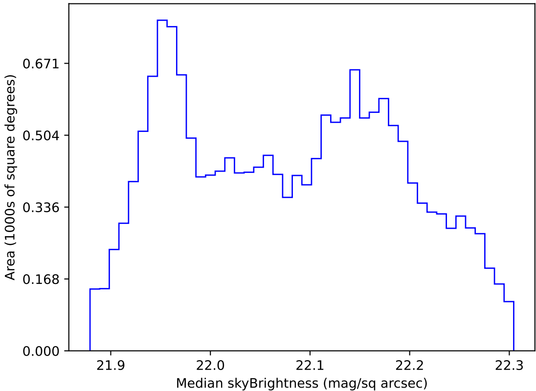
noroll_mjdp180_v3.4_10yrs WFD g band: Median skyBrightness
