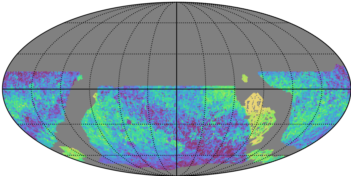
noroll_mjdp180_v3.4_10yrs WFD all bands: Median skyBrightness
