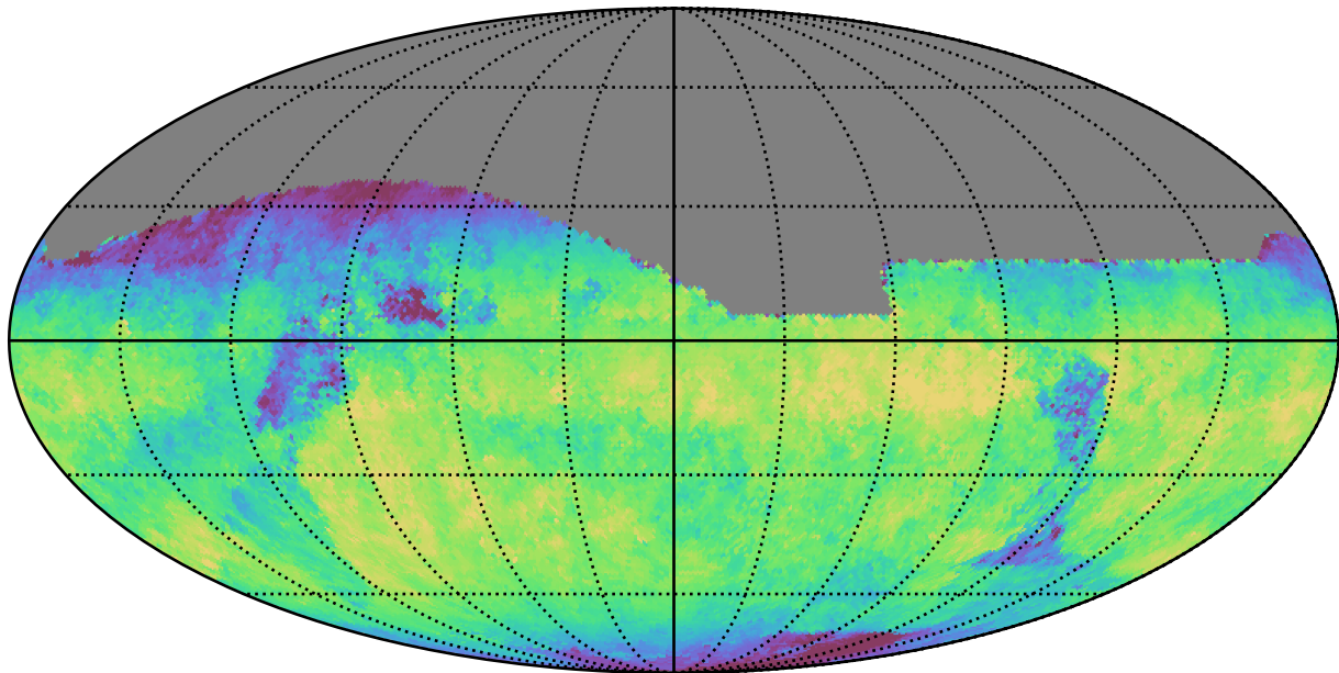
noroll_mjdp180_v3.4_10yrs All sky z band: Median skyBrightness
