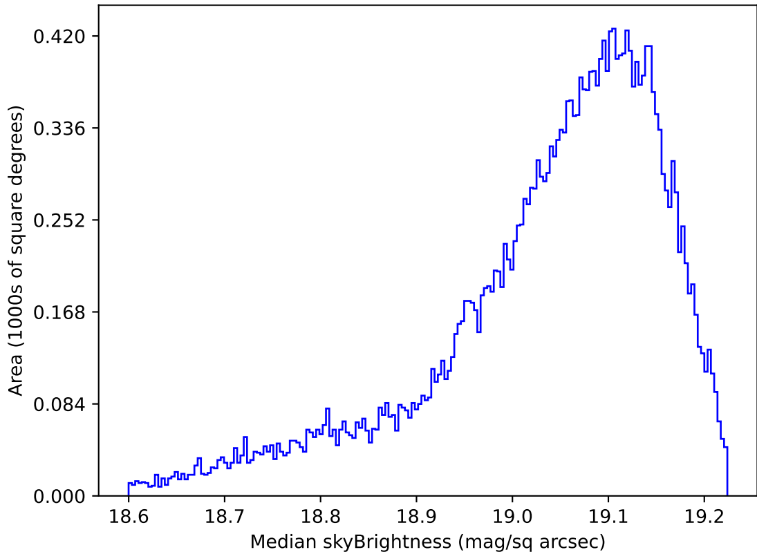
noroll_mjdp180_v3.4_10yrs All sky z band: Median skyBrightness
