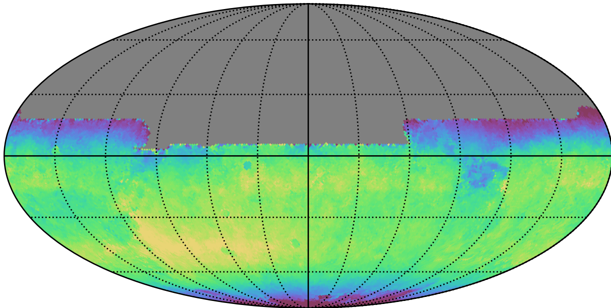
noroll_mjdp180_v3.4_10yrs All sky y band: Median skyBrightness
