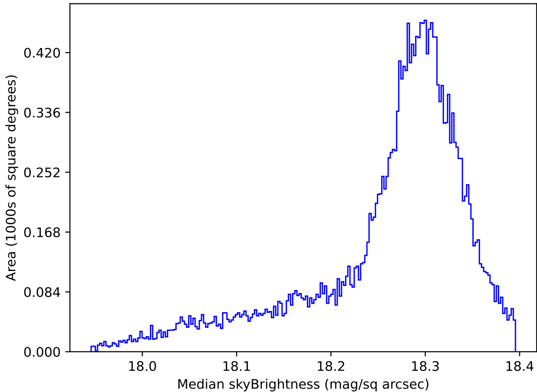
noroll_mjdp180_v3.4_10yrs All sky y band: Median skyBrightness
