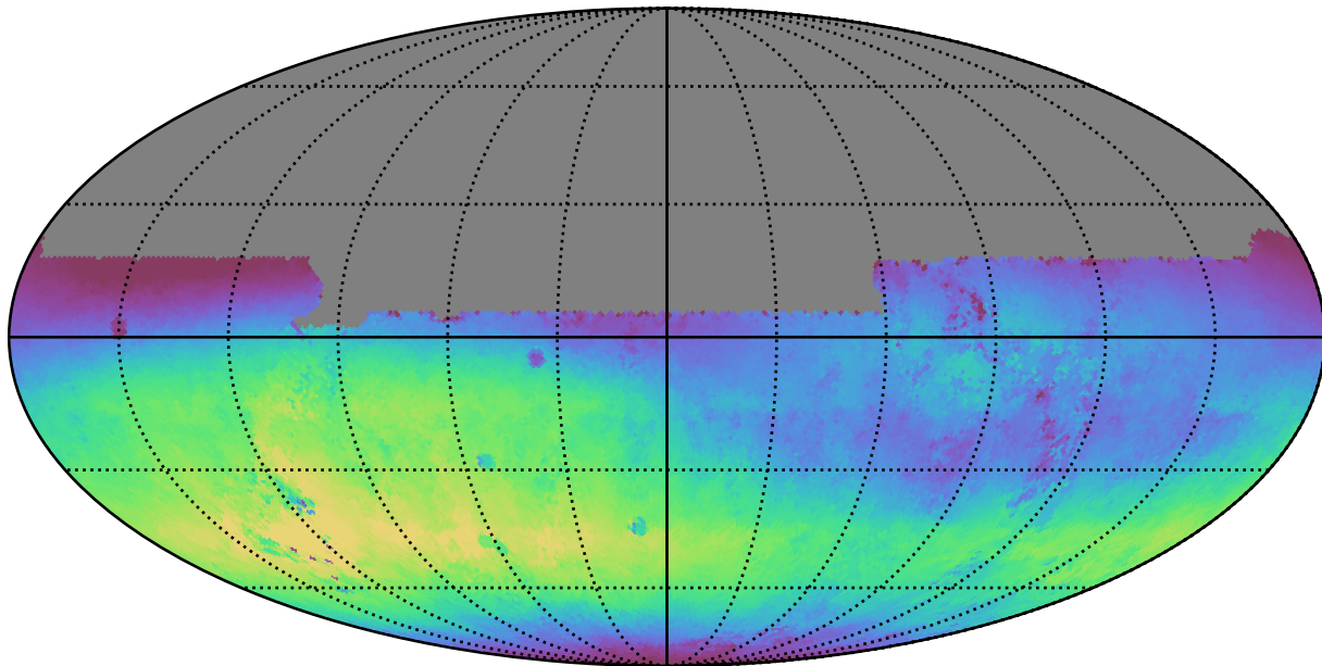
noroll_mjdp180_v3.4_10yrs All sky u band: Median skyBrightness
