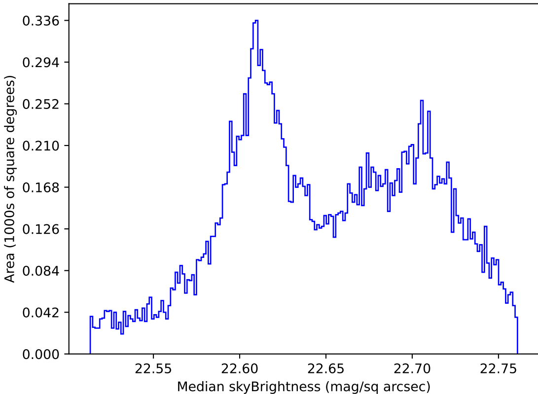
noroll_mjdp180_v3.4_10yrs All sky u band: Median skyBrightness
