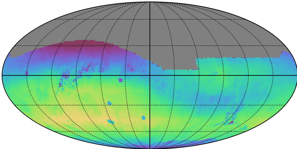
noroll_mjdp180_v3.4_10yrs All sky r band: Median skyBrightness
