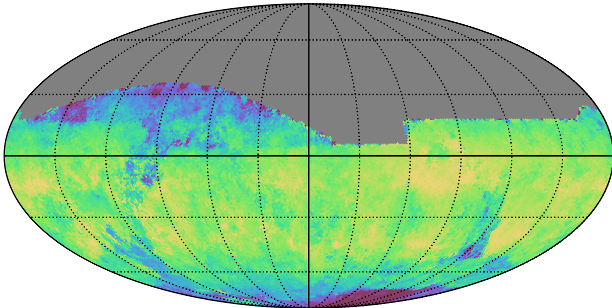
noroll_mjdp180_v3.4_10yrs All sky i band: Median skyBrightness
