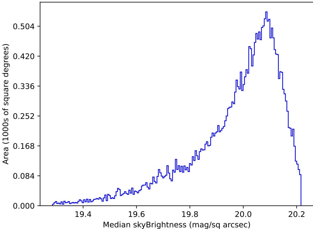
noroll_mjdp180_v3.4_10yrs All sky i band: Median skyBrightness
