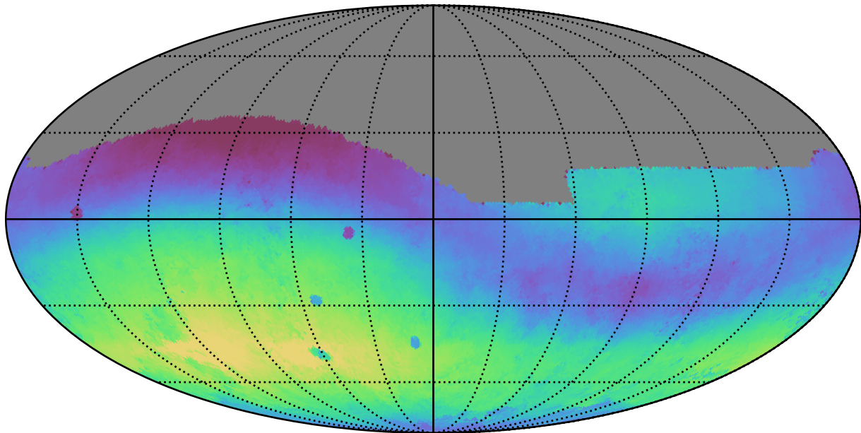
noroll_mjdp180_v3.4_10yrs All sky g band: Median skyBrightness
