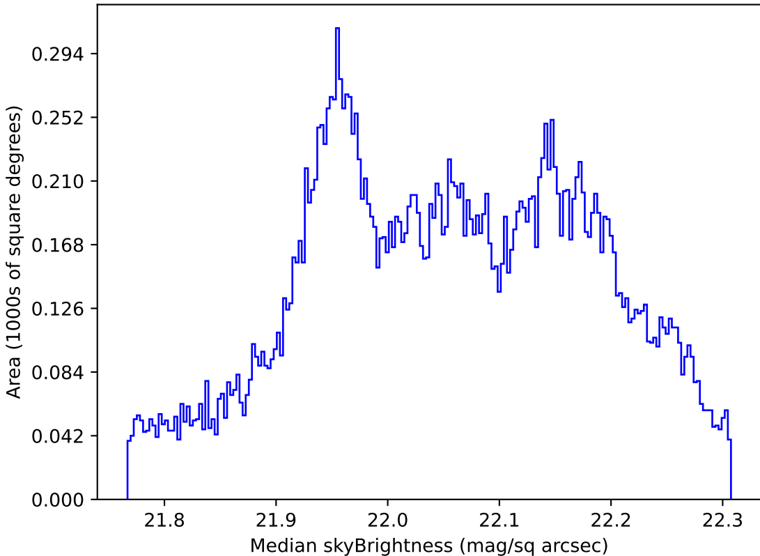
noroll_mjdp180_v3.4_10yrs All sky g band: Median skyBrightness
