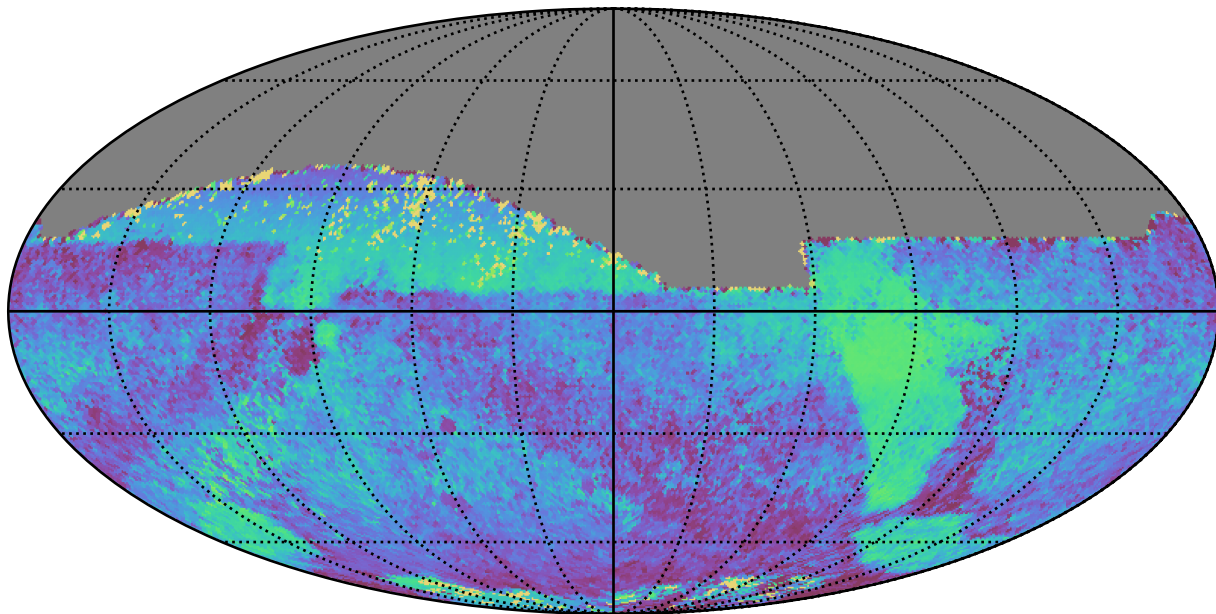
noroll_mjdp180_v3.4_10yrs All sky all bands: Median skyBrightness
