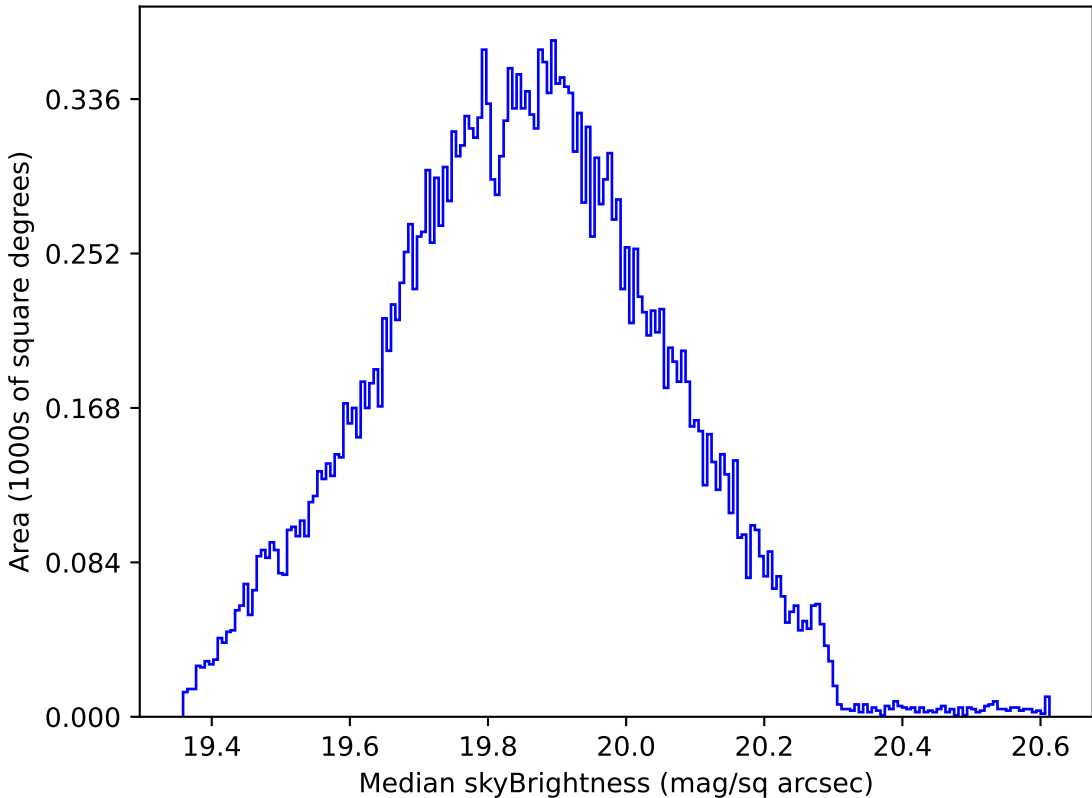
noroll_mjdp180_v3.4_10yrs All sky all bands: Median skyBrightness
