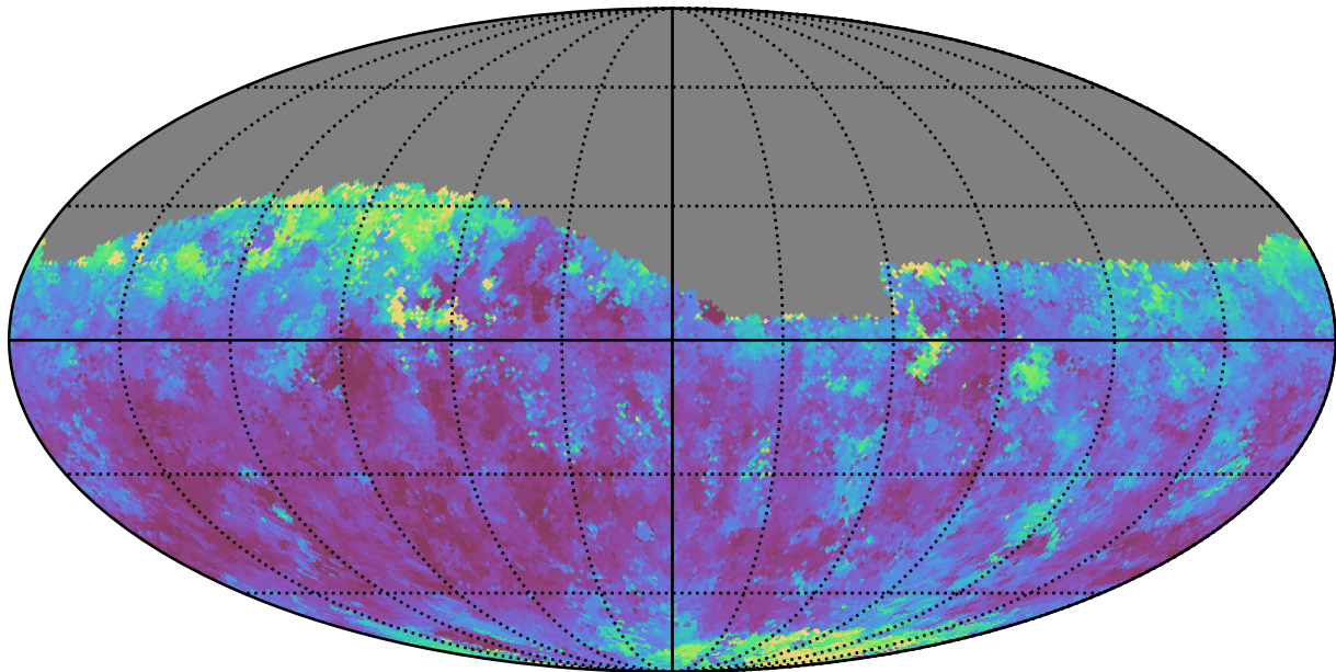
noroll_mjdp180_v3.4_10yrs Yr 1 z band: Median seeingGeom
