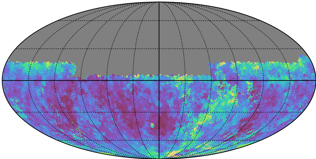
noroll_mjdp180_v3.4_10yrs Yr 1 y band: Median seeingGeom
