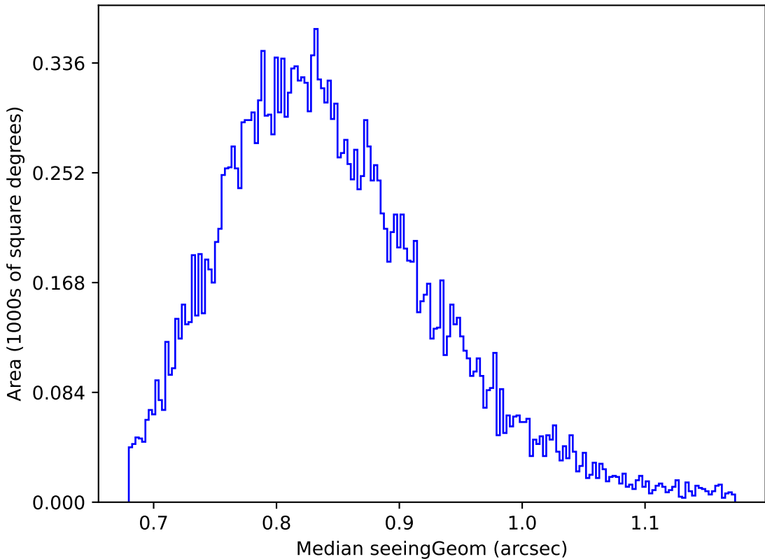
noroll_mjdp180_v3.4_10yrs Yr 1 y band: Median seeingGeom
