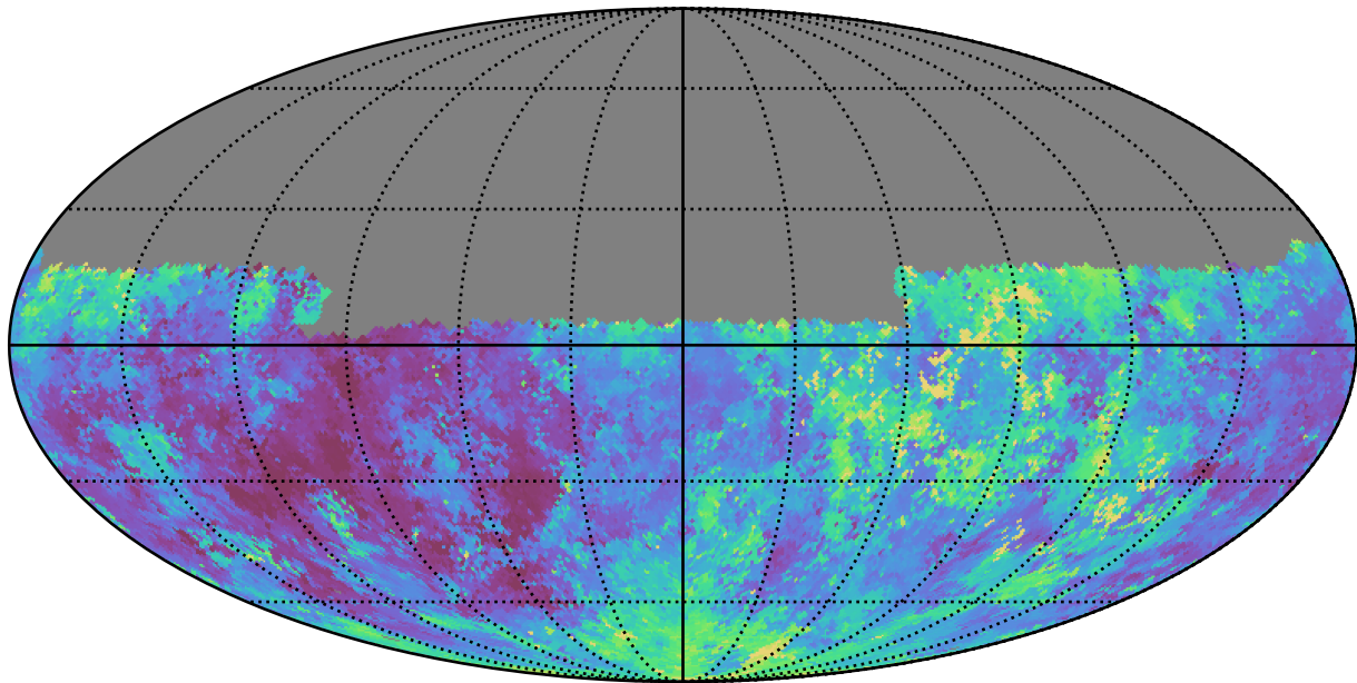
noroll_mjdp180_v3.4_10yrs Yr 1 u band: Median seeingGeom
