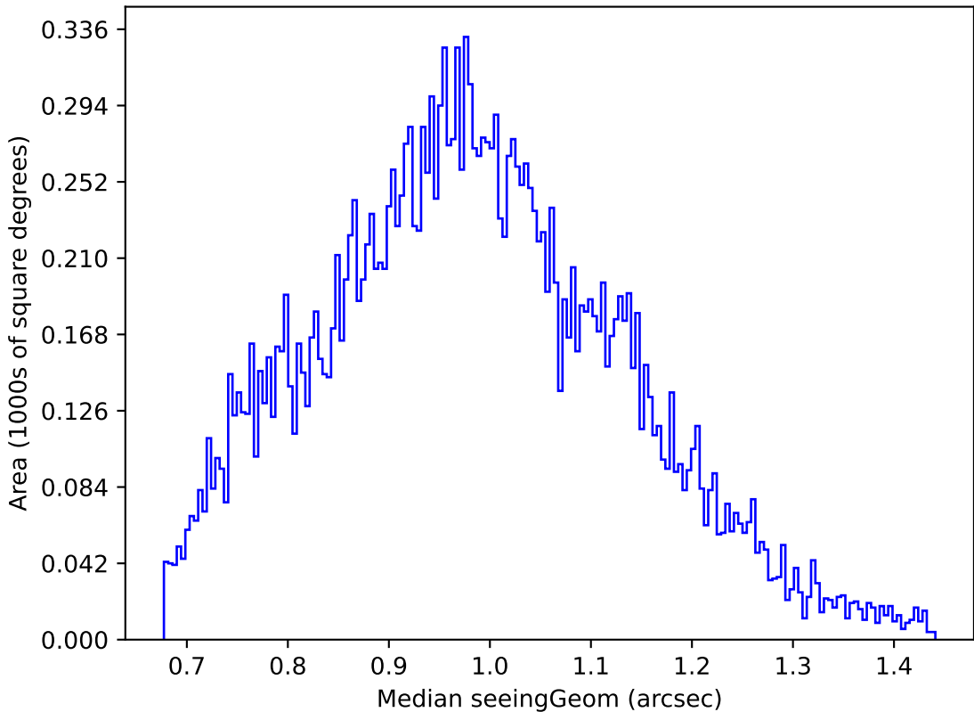
noroll_mjdp180_v3.4_10yrs Yr 1 u band: Median seeingGeom
