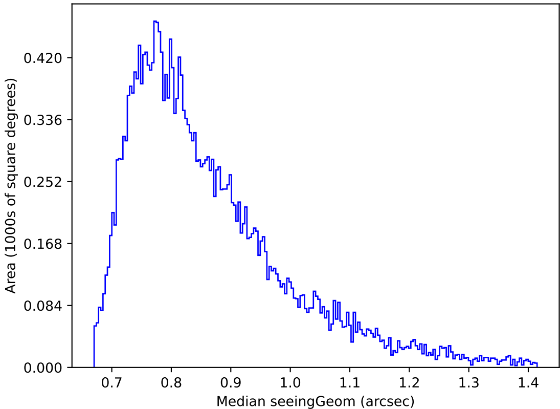
noroll_mjdp180_v3.4_10yrs Yr 1 r band: Median seeingGeom
