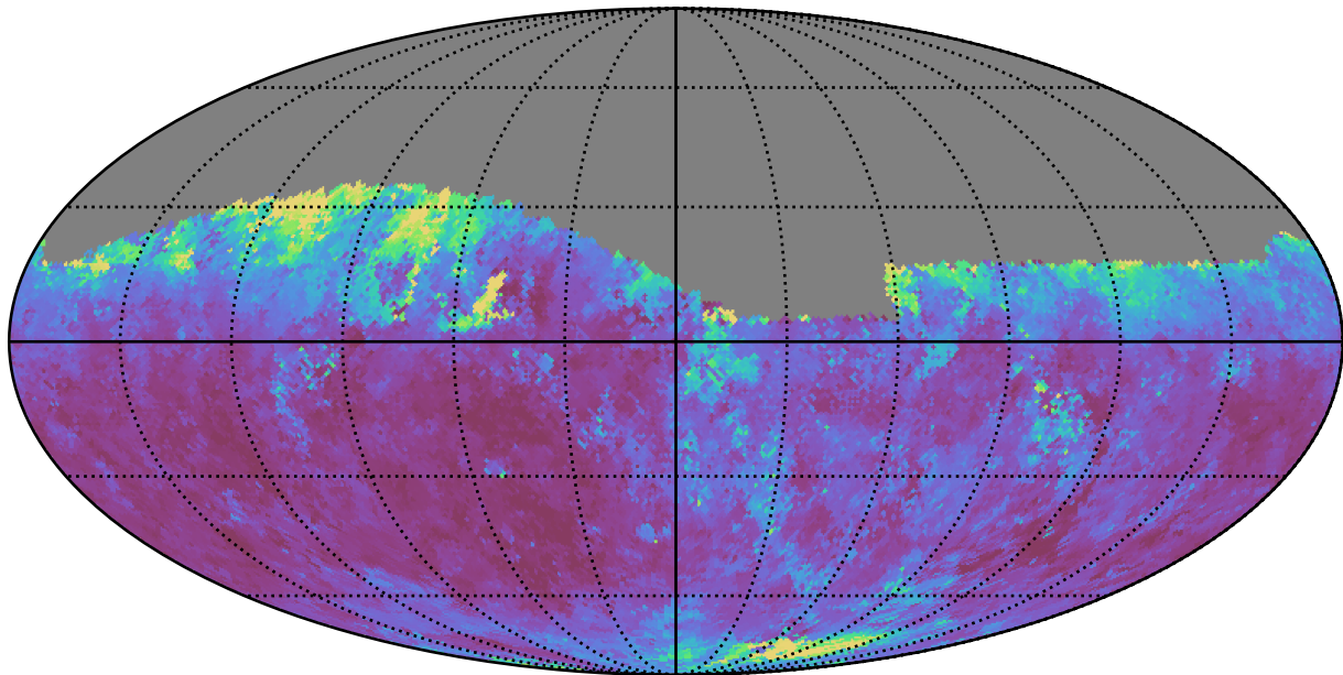
noroll_mjdp180_v3.4_10yrs Yr 1 i band: Median seeingGeom
