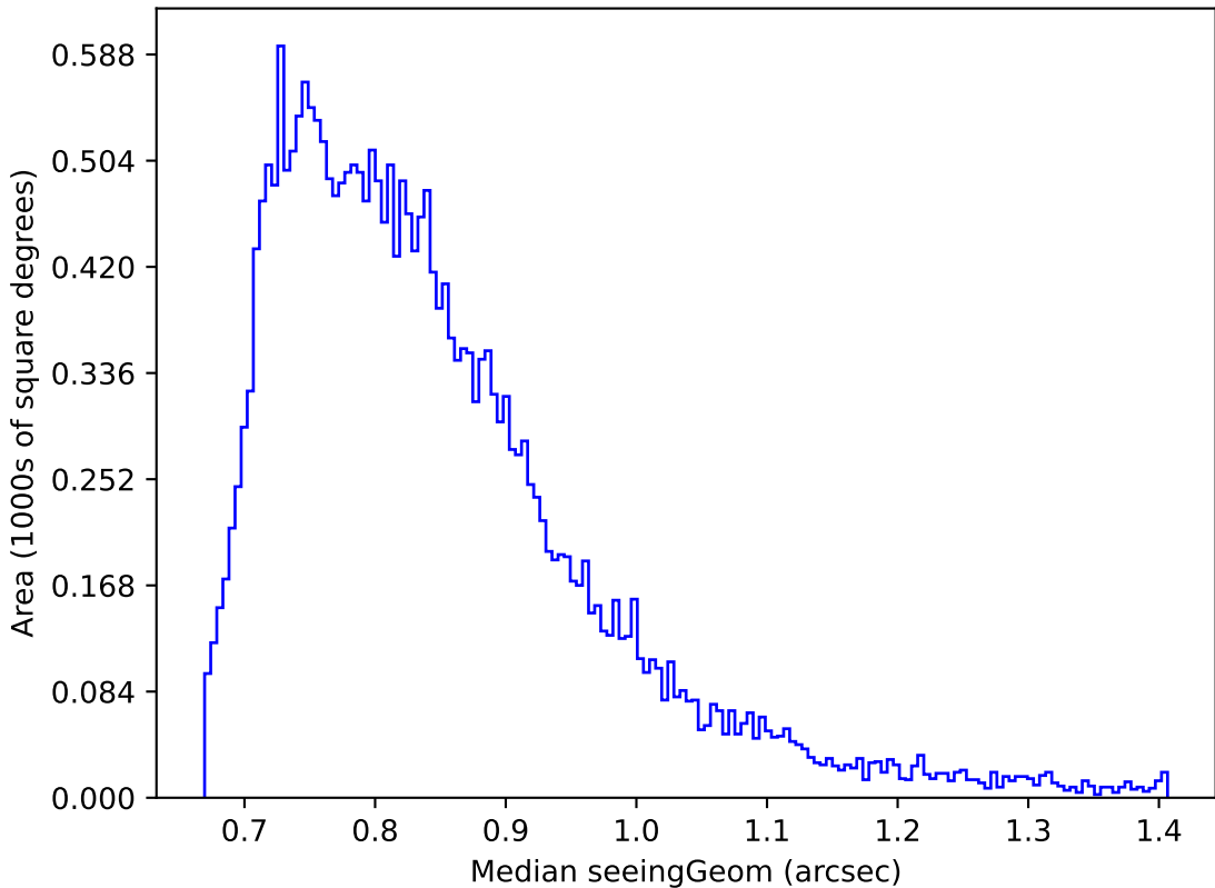
noroll_mjdp180_v3.4_10yrs Yr 1 i band: Median seeingGeom
