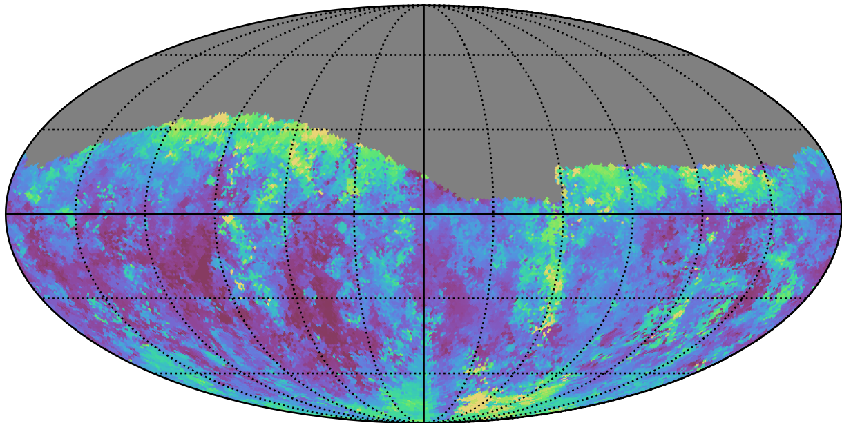
noroll_mjdp180_v3.4_10yrs Yr 1 g band: Median seeingGeom
