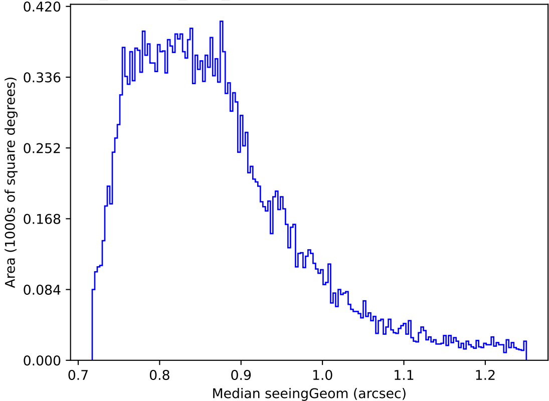
noroll_mjdp180_v3.4_10yrs Yr 1 all bands: Median seeingGeom
