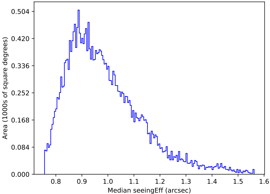
noroll_mjdp180_v3.4_10yrs Yr 1 z band: Median seeingEff
