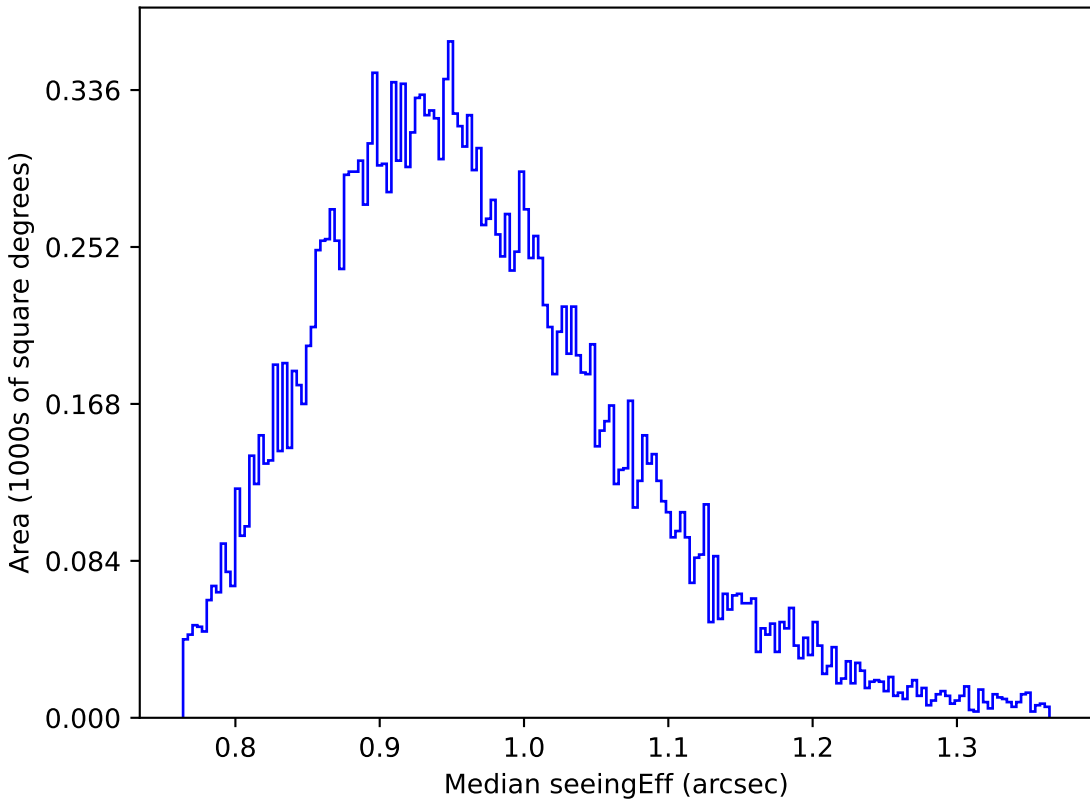
noroll_mjdp180_v3.4_10yrs Yr 1 y band: Median seeingEff
