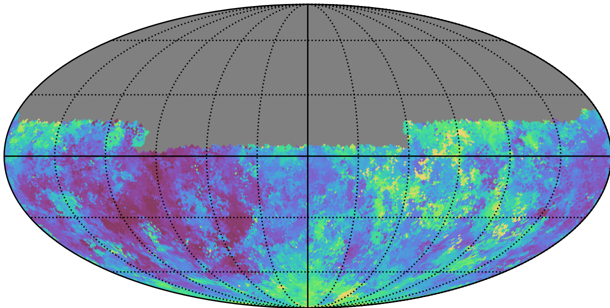
noroll_mjdp180_v3.4_10yrs Yr 1 u band: Median seeingEff
