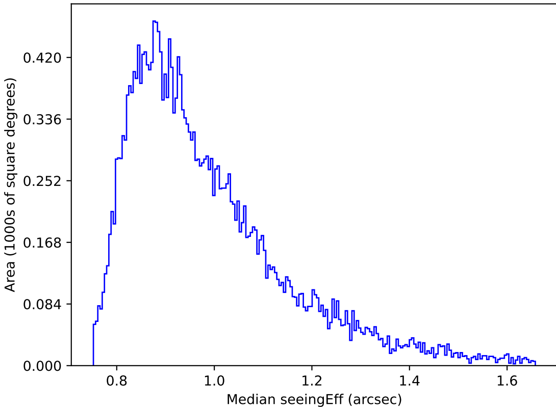
noroll_mjdp180_v3.4_10yrs Yr 1 r band: Median seeingEff
