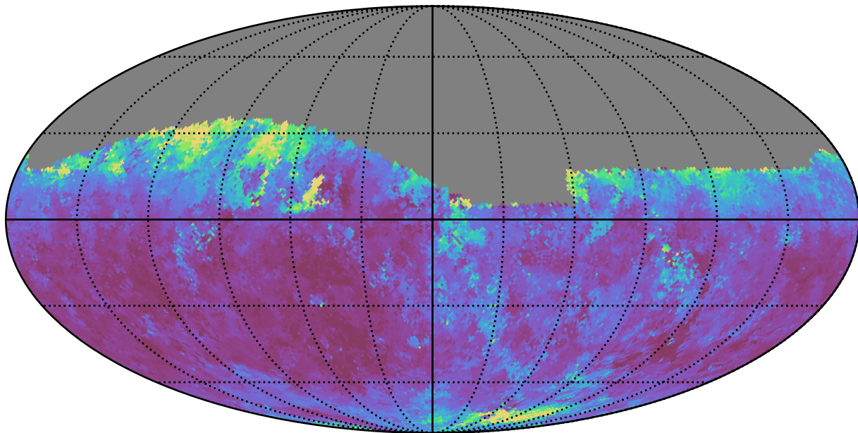
noroll_mjdp180_v3.4_10yrs Yr 1 i band: Median seeingEff
