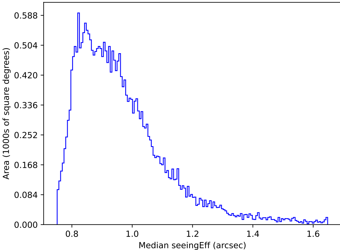
noroll_mjdp180_v3.4_10yrs Yr 1 i band: Median seeingEff
