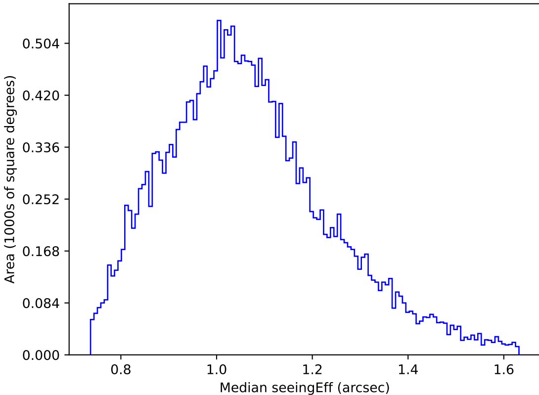
noroll_mjdp180_v3.4_10yrs Yr 1 g band: Median seeingEff
