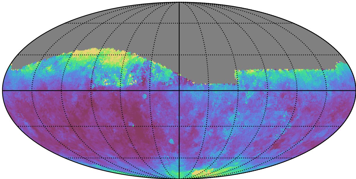
noroll_mjdp180_v3.4_10yrs Yr 1 all bands: Median seeingEff
