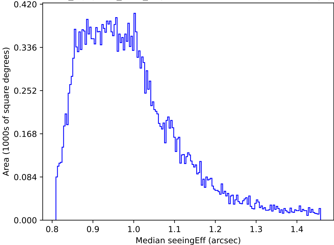
noroll_mjdp180_v3.4_10yrs Yr 1 all bands: Median seeingEff
