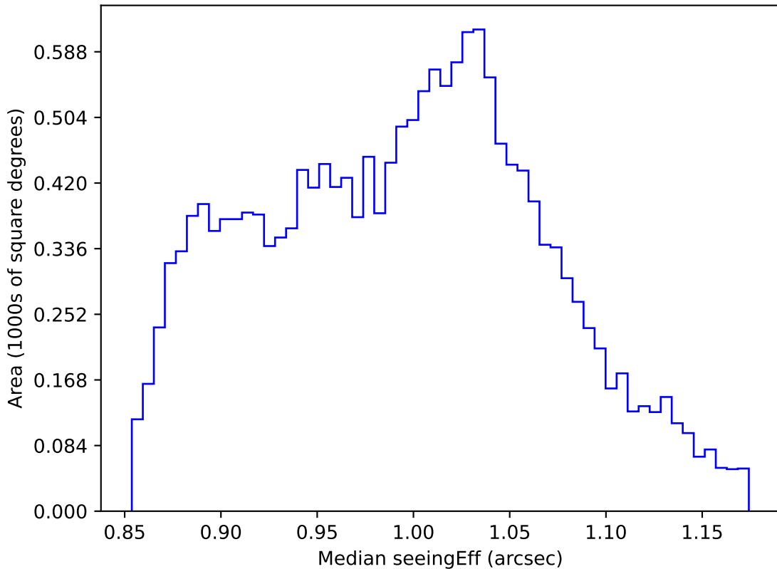
noroll_mjdp180_v3.4_10yrs WFD z band: Median seeingEff
