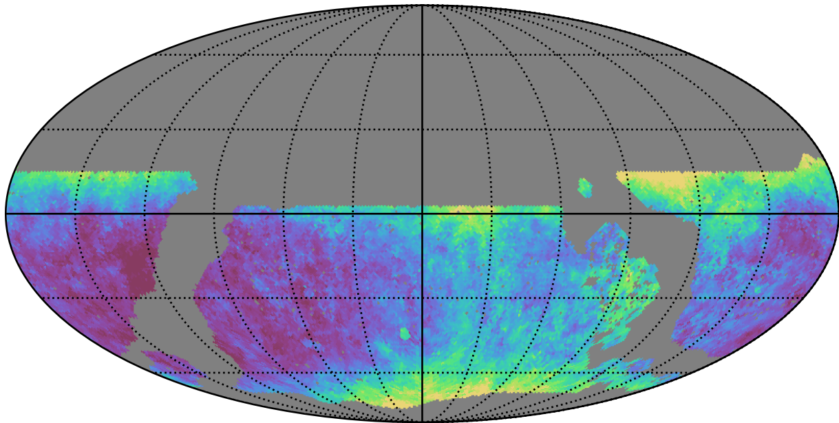
noroll_mjdp180_v3.4_10yrs WFD y band: Median seeingEff
