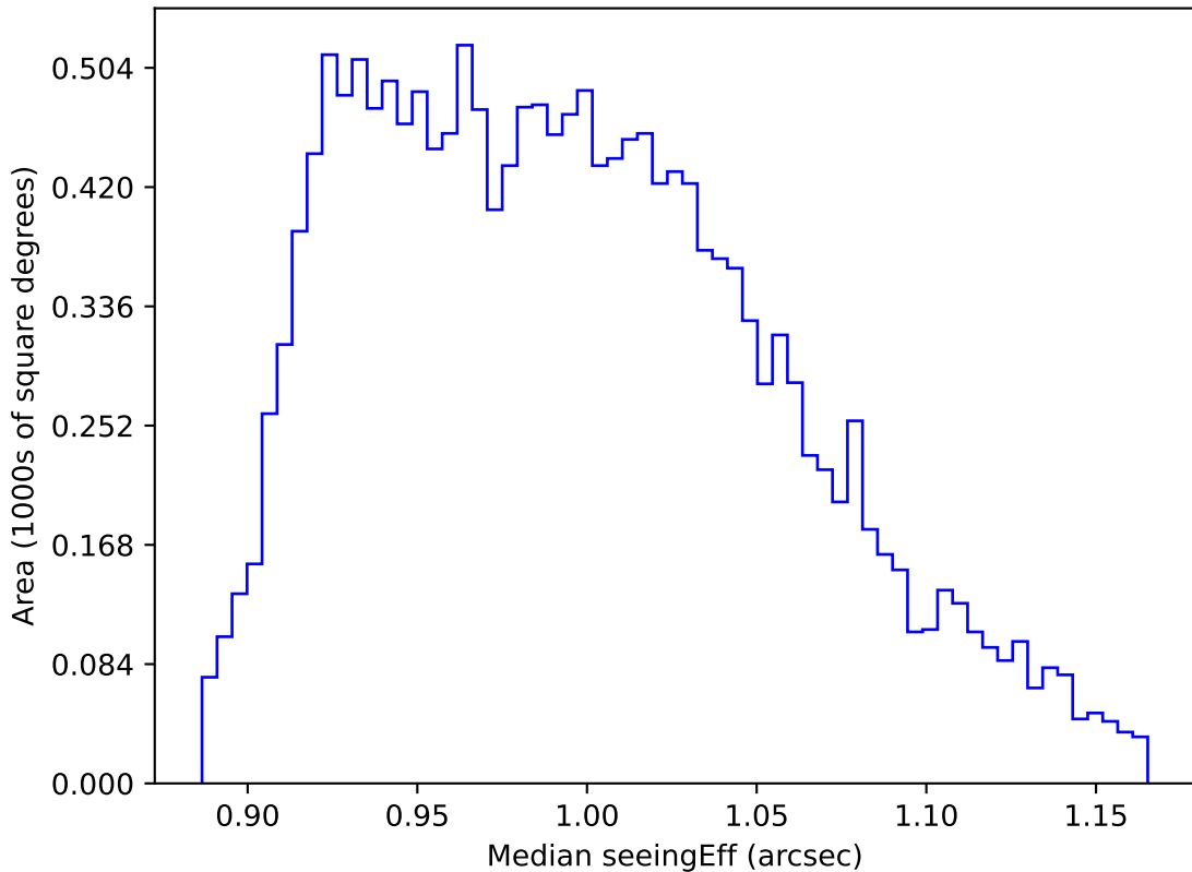
noroll_mjdp180_v3.4_10yrs WFD y band: Median seeingEff
