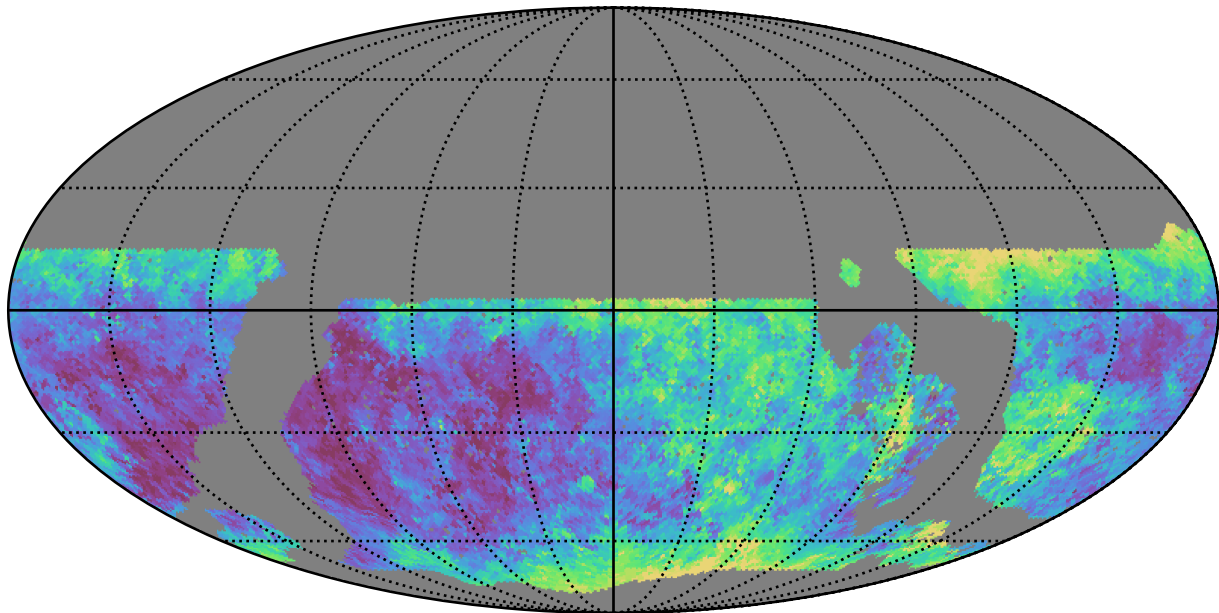
noroll_mjdp180_v3.4_10yrs WFD u band: Median seeingEff
