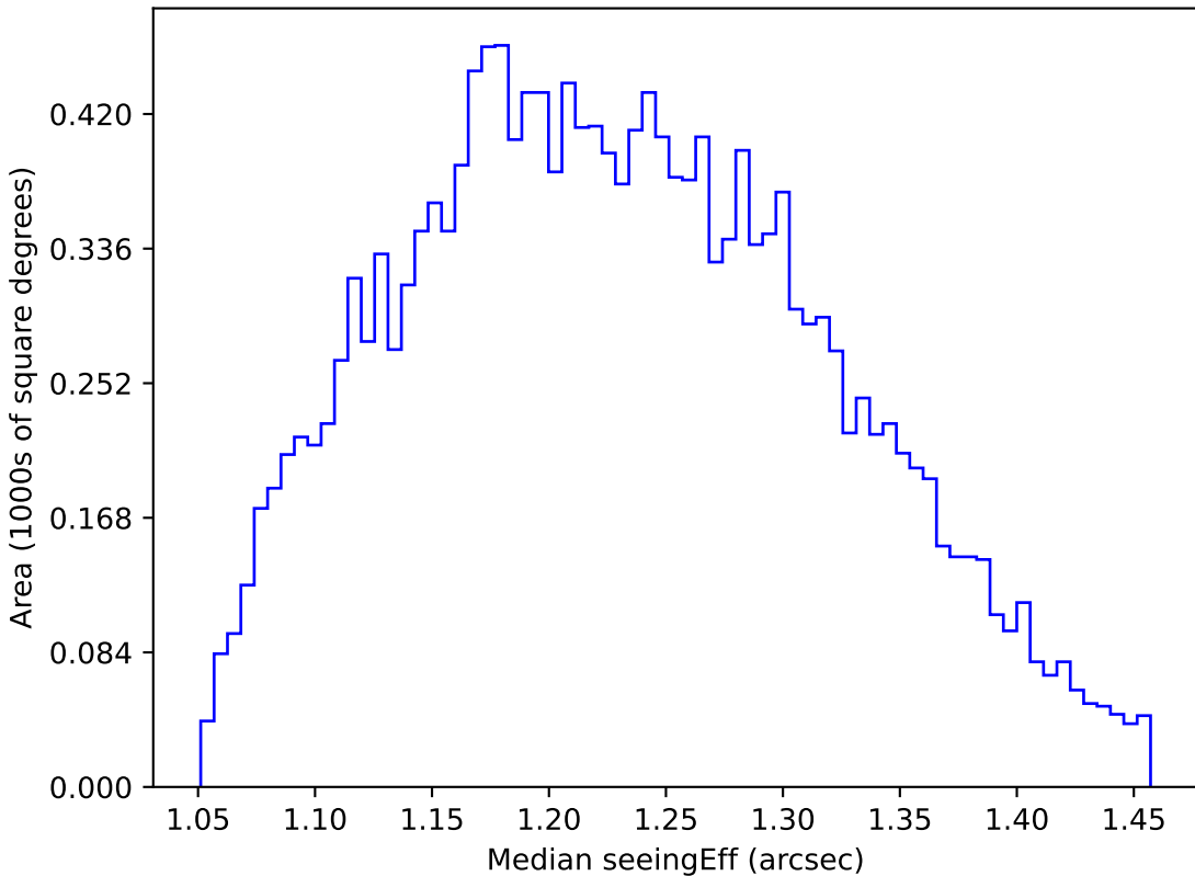
noroll_mjdp180_v3.4_10yrs WFD u band: Median seeingEff
