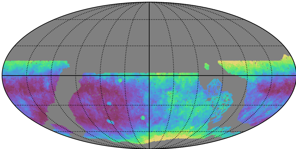
noroll_mjdp180_v3.4_10yrs WFD r band: Median seeingEff
